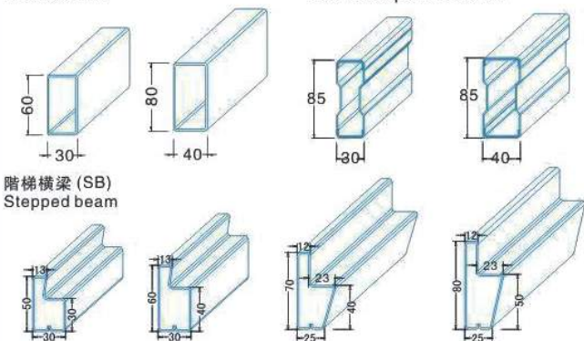
方通橫梁 (BB) Boxed beam
