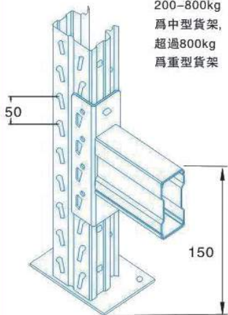
方通橫梁 (BB) Boxed beam
